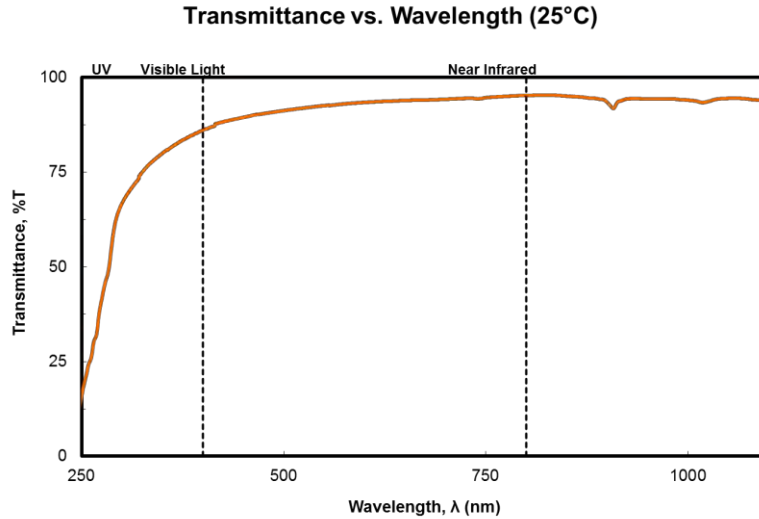
Figure 1. % Transmittance versus air, 2mm thickness
